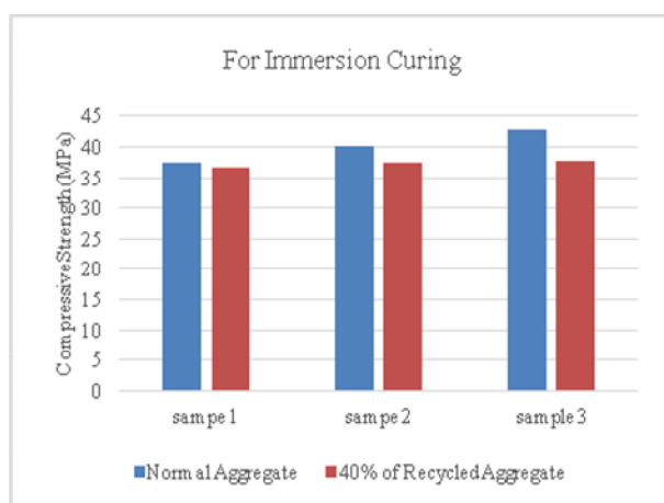
Figure 2: Shows the Compressive Strength Comparison between Concrete with Normal Aggregate and Concrete with 40% Recycled Aggregate using Immersion Curing
