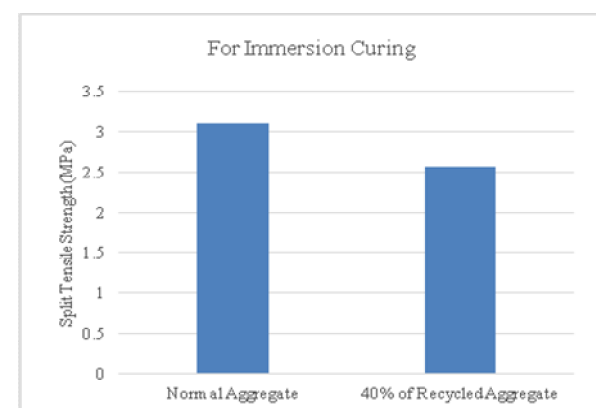
Figure 5: Shows the Spilt Tensile Strength Comparison between Concrete with Normal Aggregate and Concrete with 40% Recycled Aggregate using Immersion Curing
