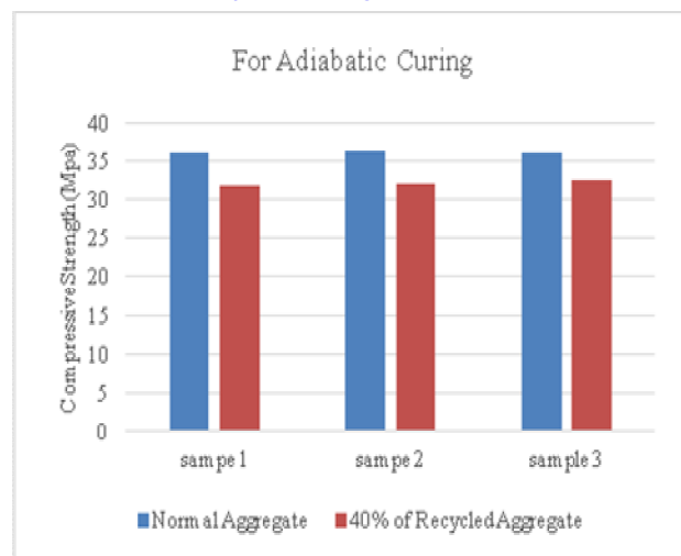
Figure 3: Shows the Compressive Strength Comparison between Concrete with Normal Aggregate and Concrete with 40% Recycled Aggregate using Adiabatic Curing
