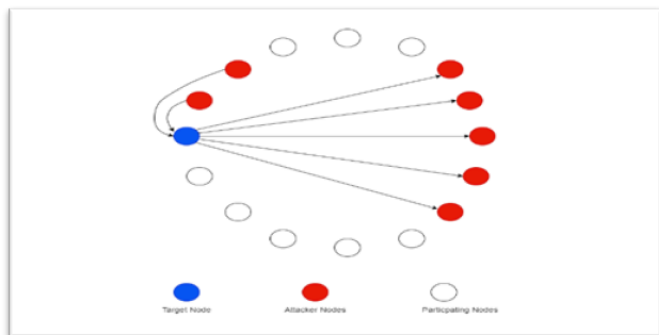
Figure.2 Eclipse Attack
