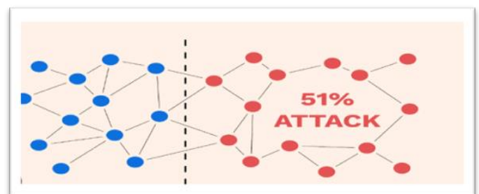
Figure.1 51% Attacks
