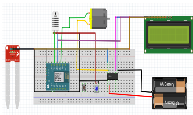
Fig.1. Circuit diagram of our proposal system
